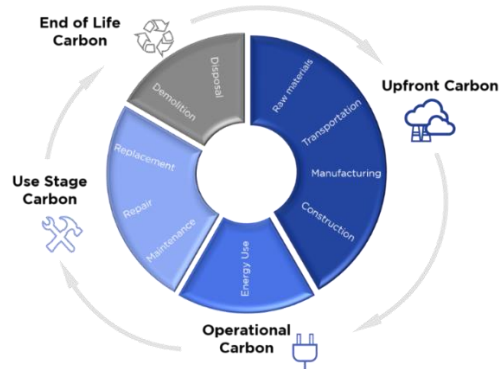
Figure 15 - The Carbon Cycle
