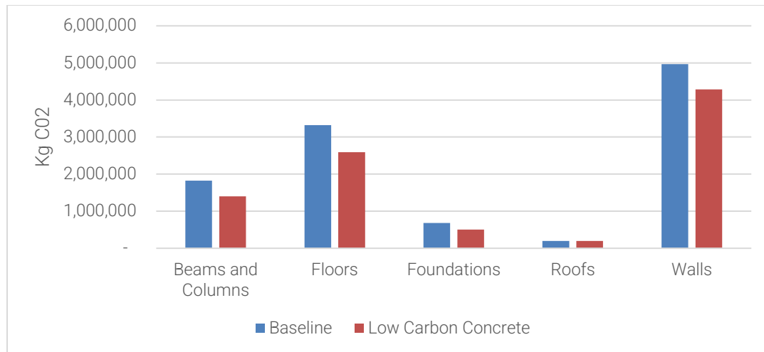
Figure 18 – Low Carbon Concrete – 30-40% SCM and GUL
