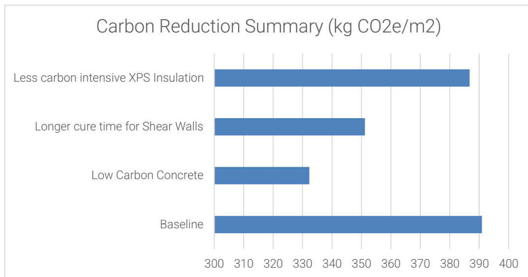
Figure 19– Embodied Carbon Reduction Summary Graph
